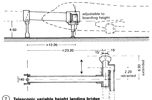
7 Telescopic variable height landing bridge
